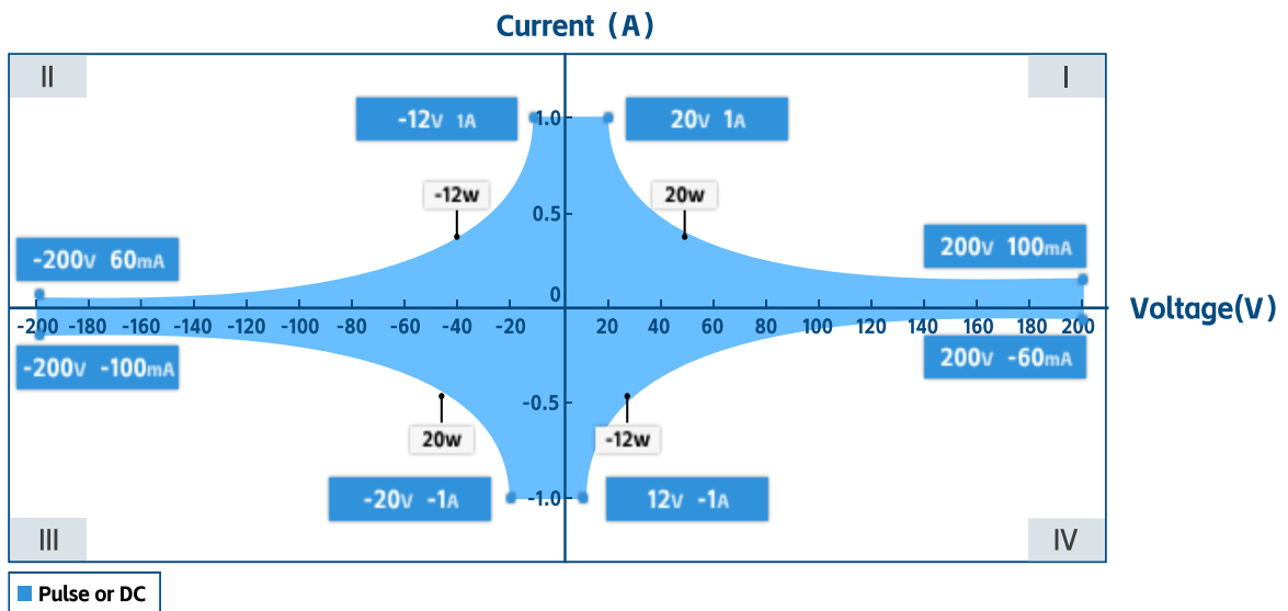
DC I-V Output Capability
