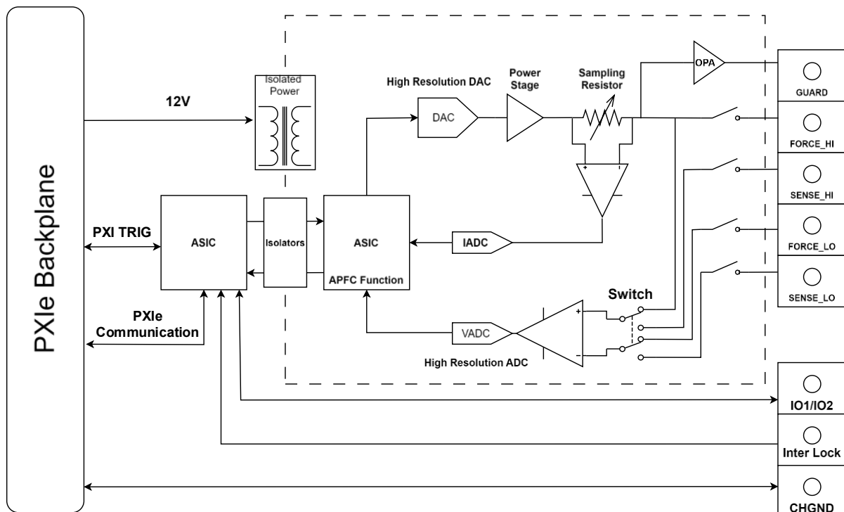
S2013C Block Diagram
