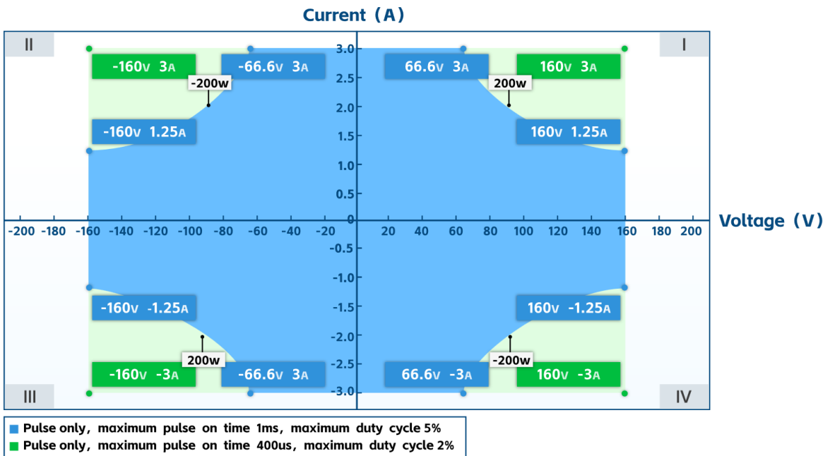
Pulse I-V Output Capability
